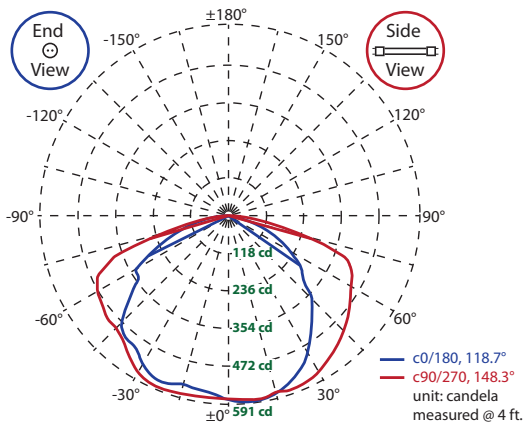
Polar Luminous Intensity
